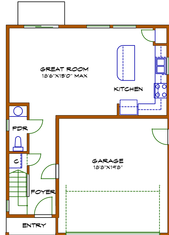
MAIN FLOOR PLAN AREA: 601 SF TOTAL AREA: 1199 SF
