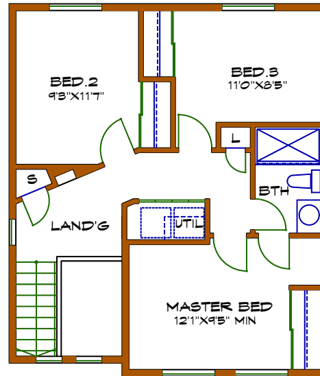
UPPER FLOOR PLAN AREA: 598 SF
