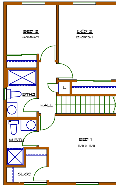
UPPER FLOOR PLAN 640 SF THIS FLOOR
